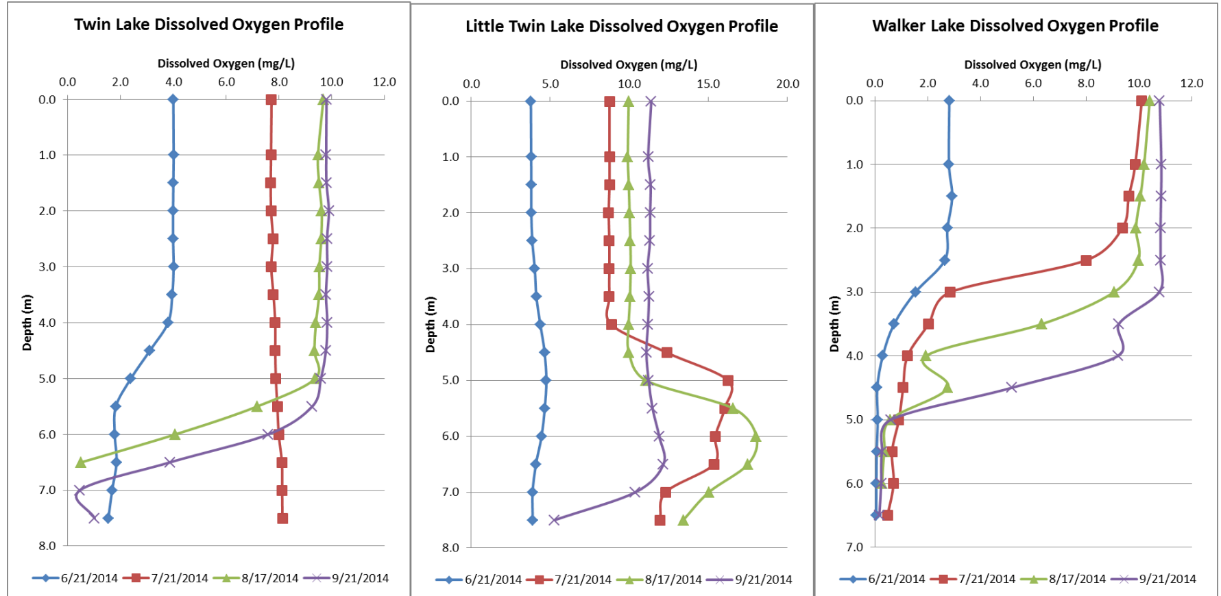
Figure 5. Dissolved Oxygen Profiles in 2014 for Big Twin Lake, Little Twin Lake and Walker Lake
