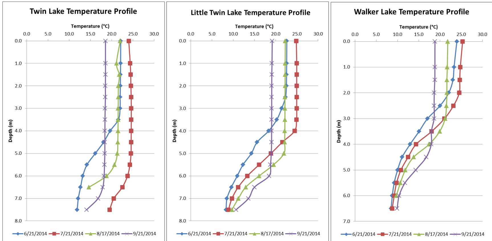
Figure 4. Temperature Profiles in 2014 for Big Twin Lake, Little Twin Lake and Walker Lake
