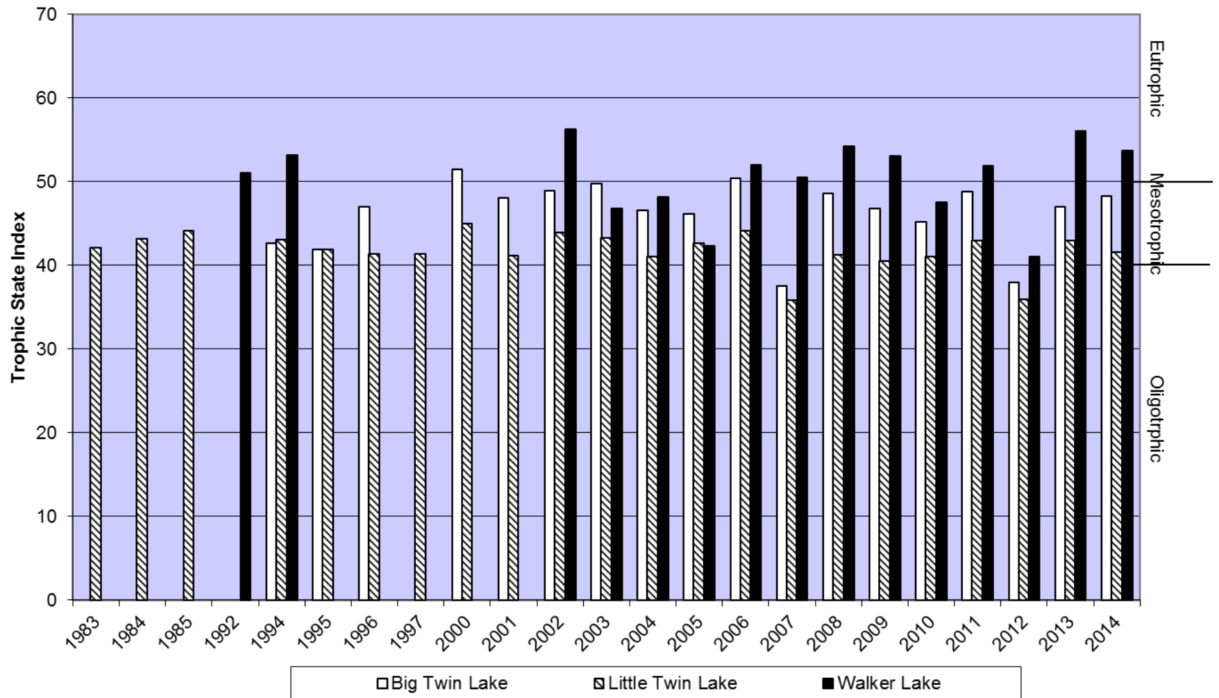
Figure 3. Comparison of Secchi Depth-Based Trophic State Index for Big Twin Lake, Little Twin Lake, and Walker Lake 1983-2014
